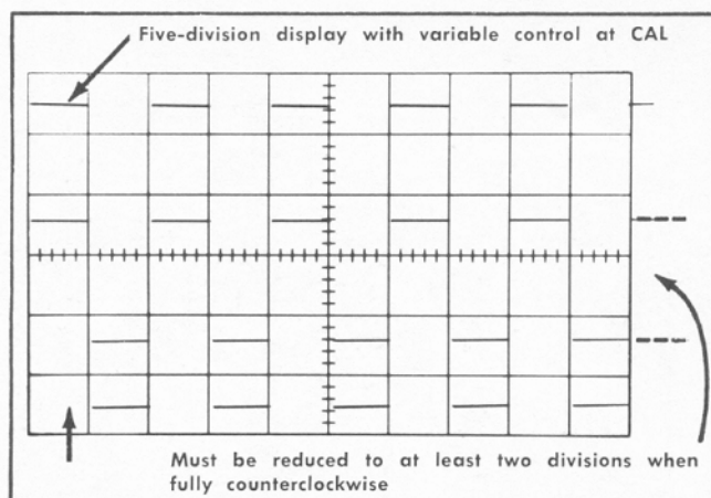
Fig. 6-22. Typical crt display showing correct VARIABLE VOLTS/DIV control range (double exposure).
