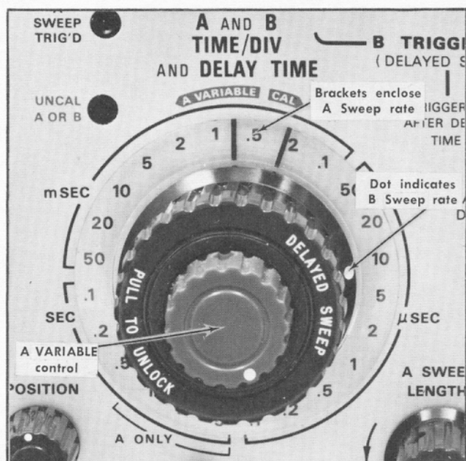
Fig. 2-8. A AND B TIME/DIV switch.
