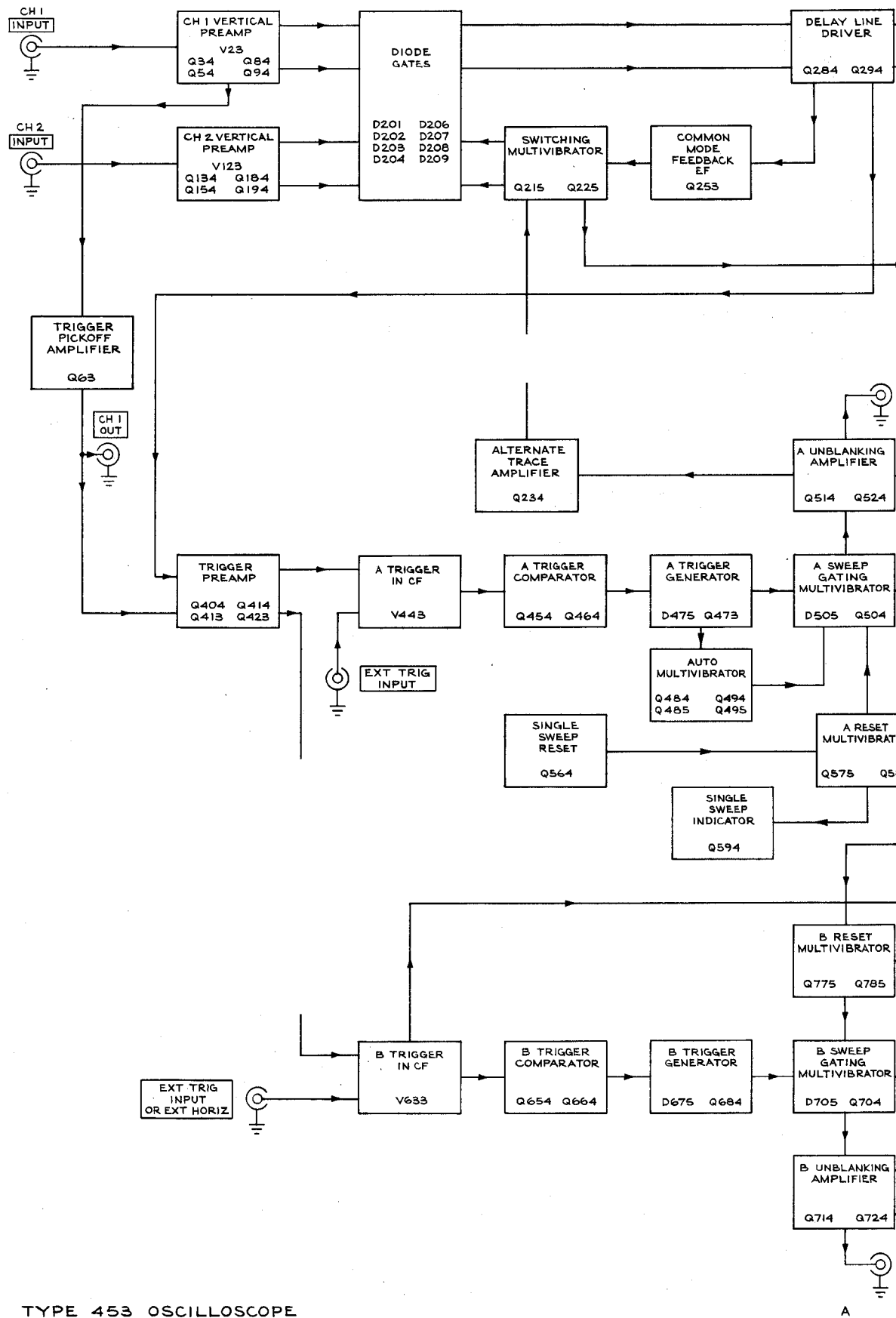
TYPE 453 OSCILLOSCOPE
