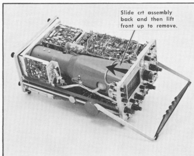
Fig. 4-2. Removing the cathode-ray tube.
