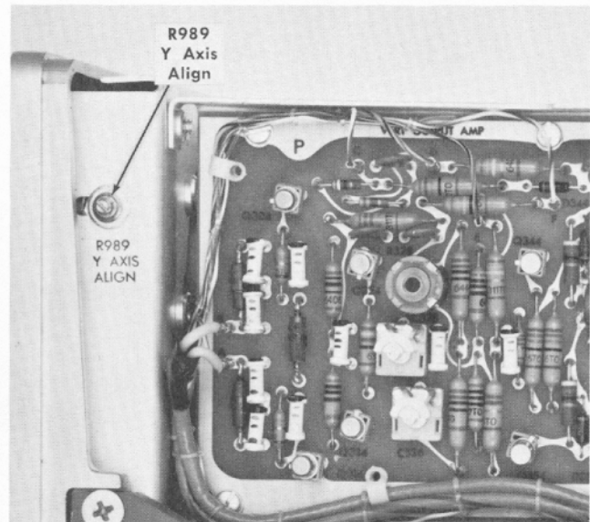
Fig. 6-16. Location of Y Axis Alignment adjustment (left side).
