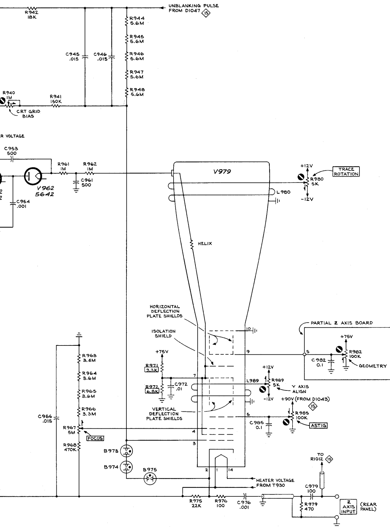
CRT CIRCUIT 16
