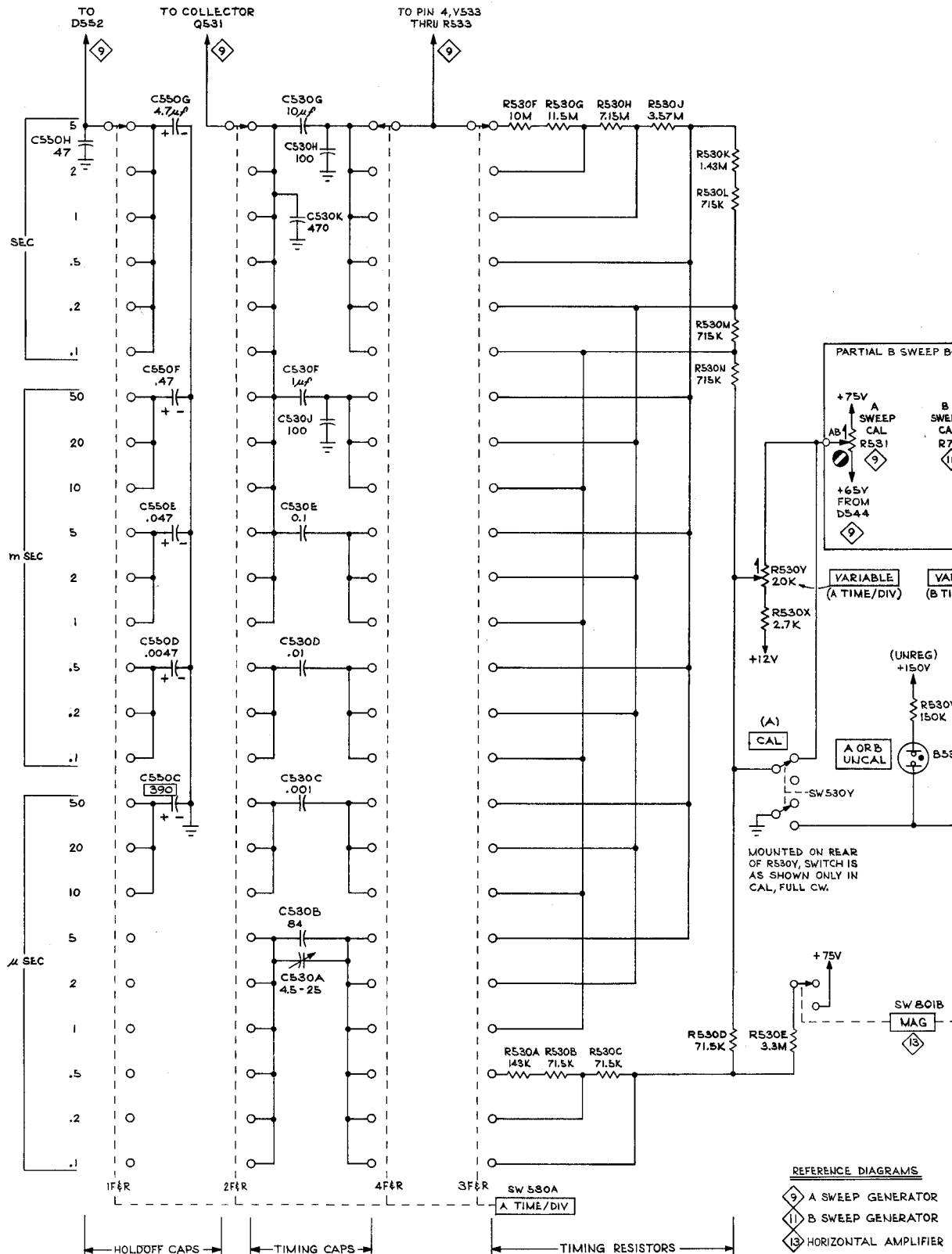
TYPE 453 OSCILLOSCOPE
