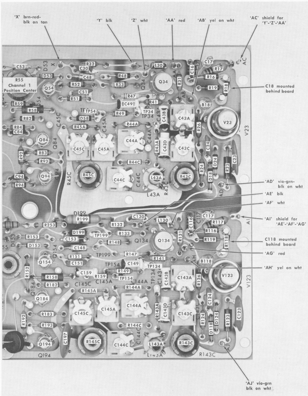
Fig. 4-6. Channel 1 and 2 Input Preamp etched-wiring board (partial Vertical Preamp board).
