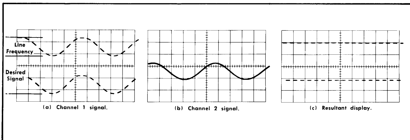
Fig. 2-26. Using the ADD feature for common-mode rejection. (a) Channel 1 signal contains desired information along with line-frequency component, (b) Channel 2 signal contains line-frequency only, (c) crt display using common-mode rejection.
