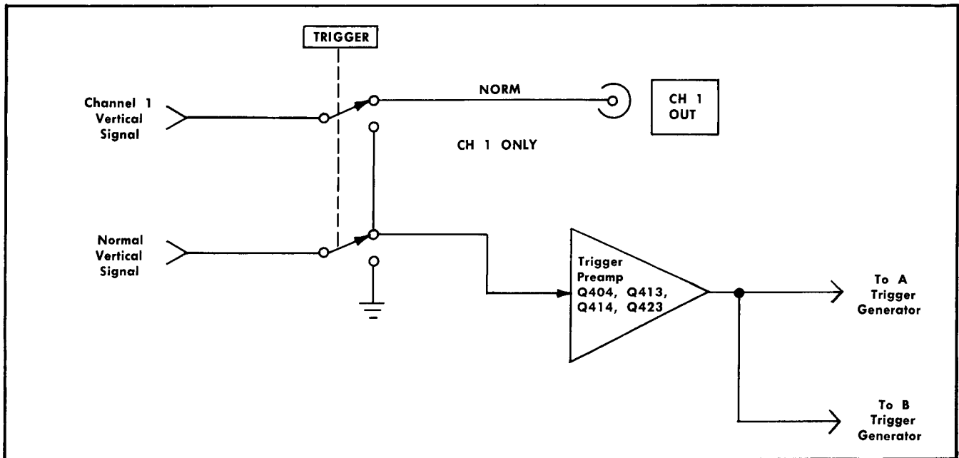
Fig. 3-5. Block diagram of Trigger Preamplifier circuit.
