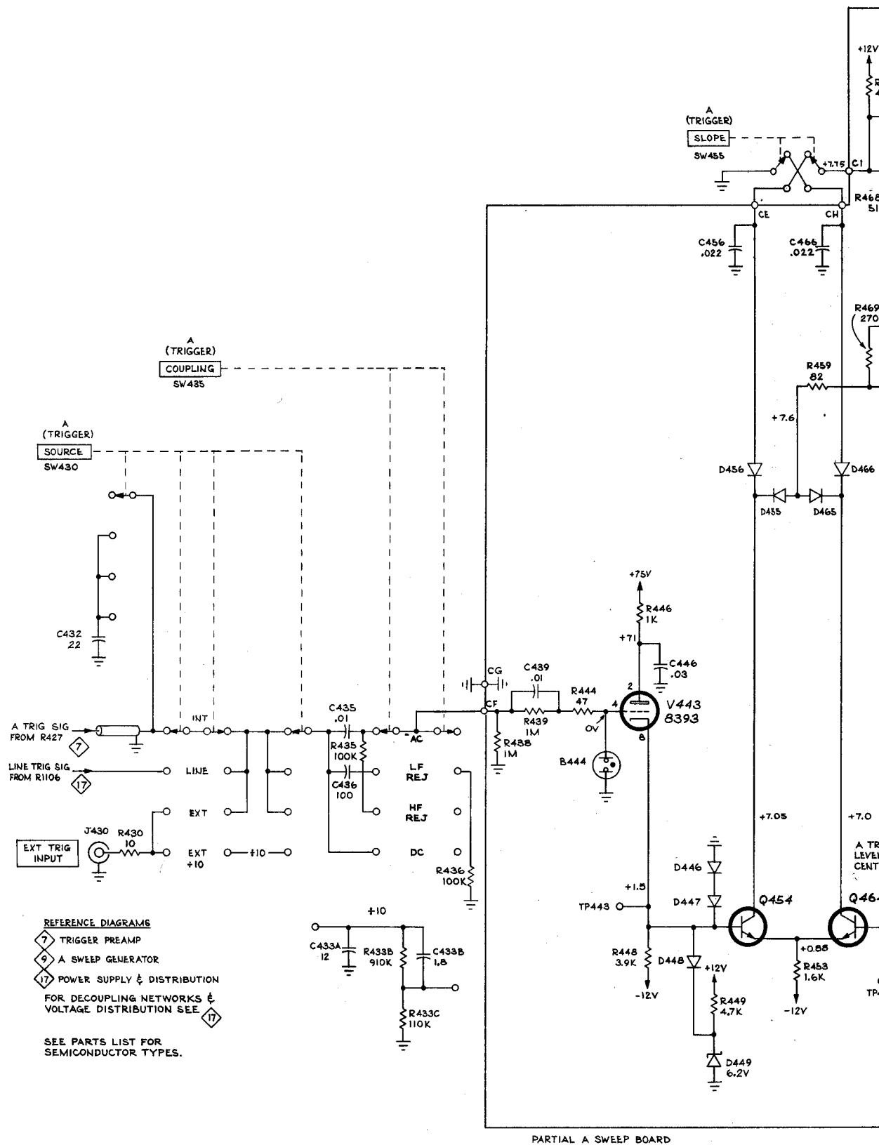
TYPE 453 OSCILLOSCOPE
