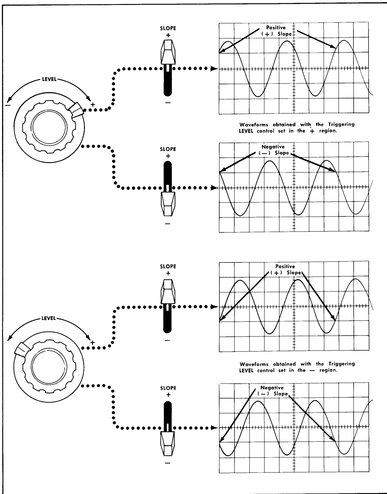
Fig. 2-7. Effects of Triggering LEVEL control and SLOPE switch.
