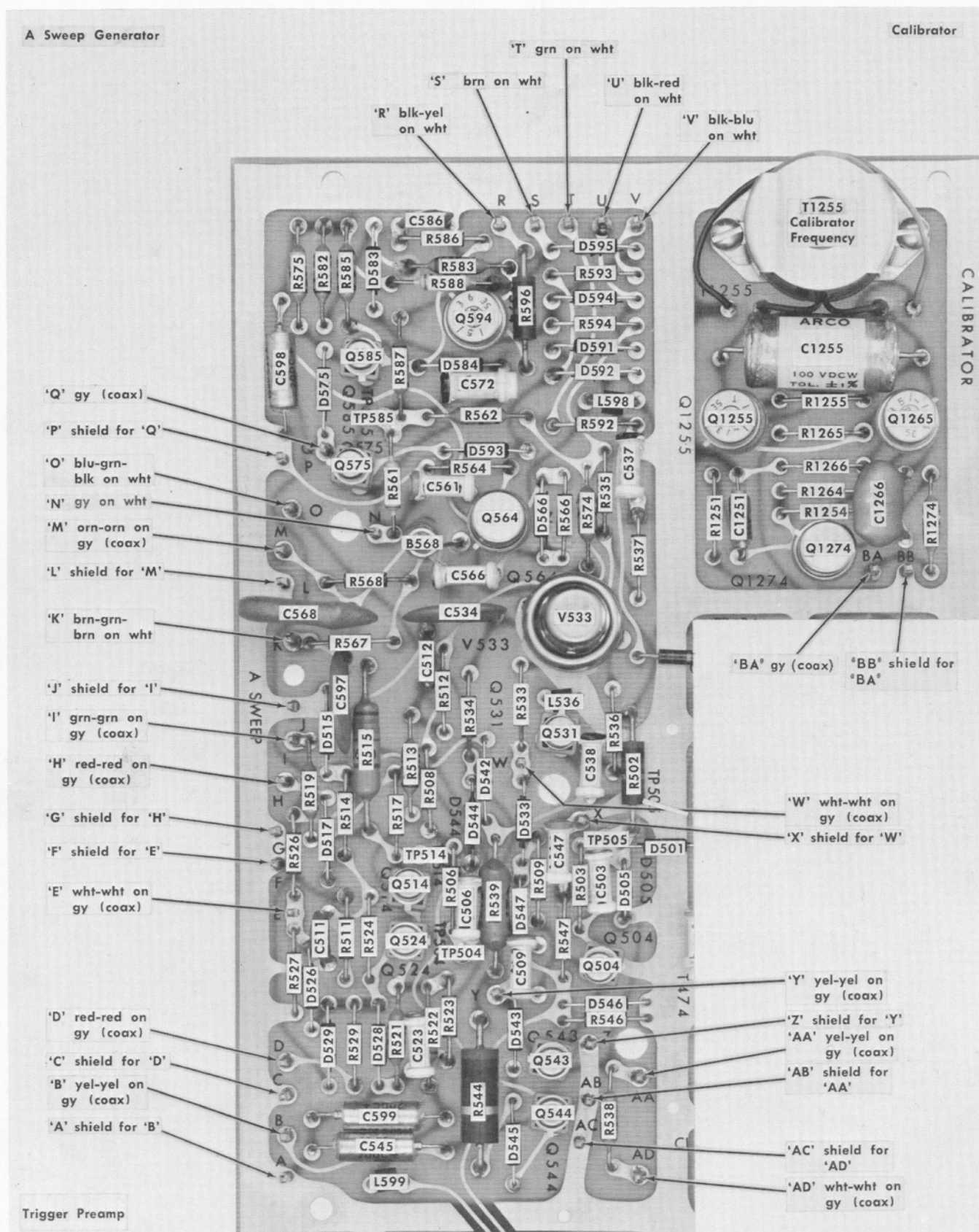
Fig. 4-7. A Sweep Generator and Calibrator etched-wiring board (partial A Sweep board).
